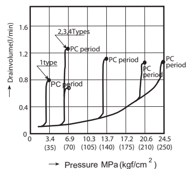
Drain volume characteristic
