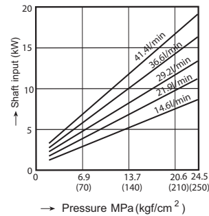
V 23 Shaft input characteristic
