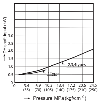
Dead head shaft input
